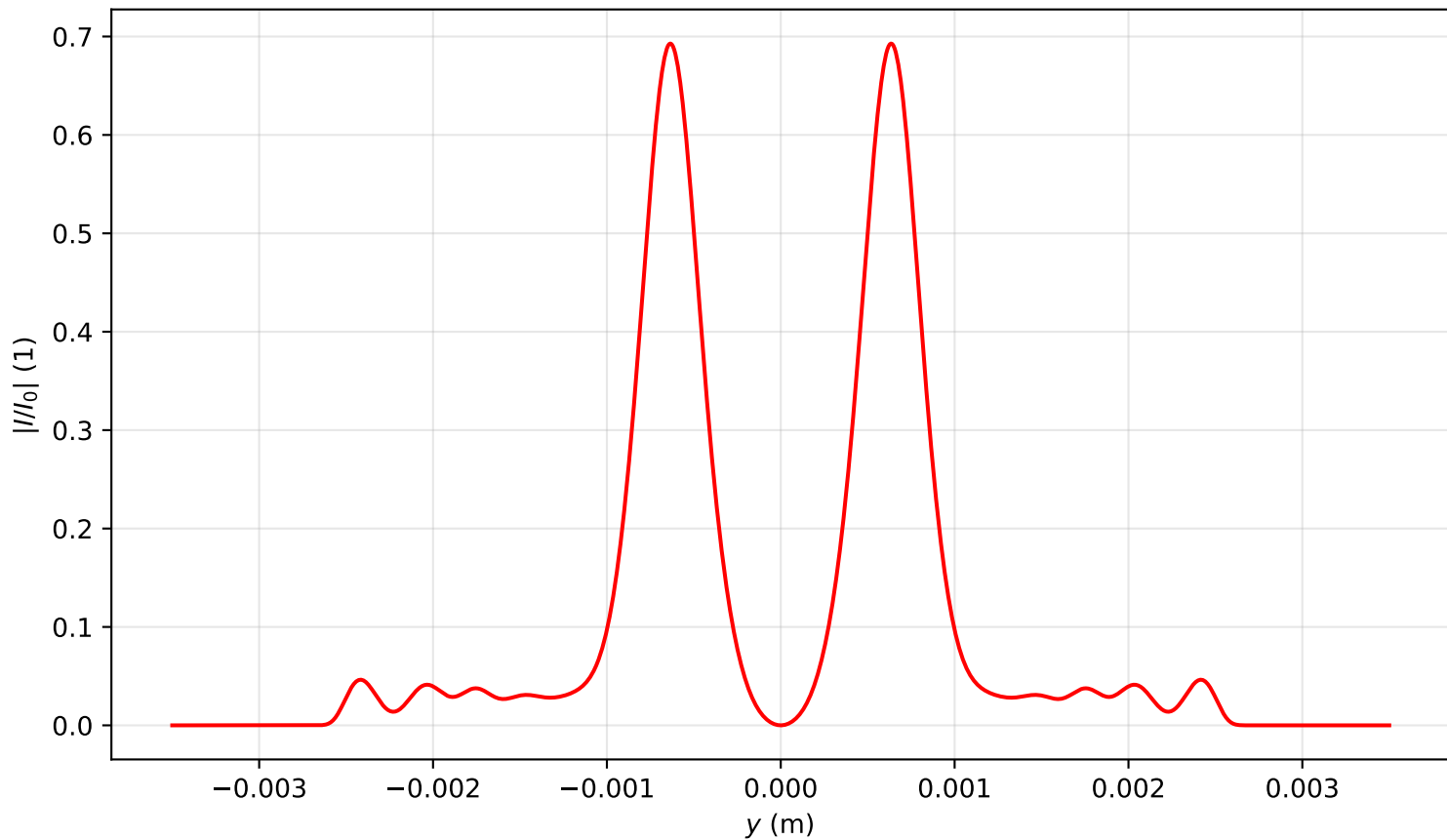
Intensity profile I(x=0, y, z=2.548)/I_0 , \text{Pin}=6.0\text{Pcr} , artificial time
